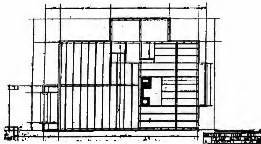
To guide the assembly of the American System-Built Houses, Wright's office prepared floor plans, elevations, sections, framing diagrams, and other details for each individual design in the catalogue. The examples above are for the design used in the Burhans-Ellinwood & Company Model House.
